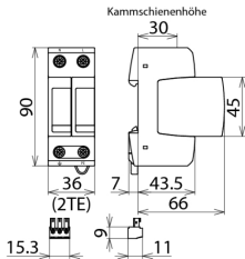
Dimensions DG M TT2P CI275 NL FM
